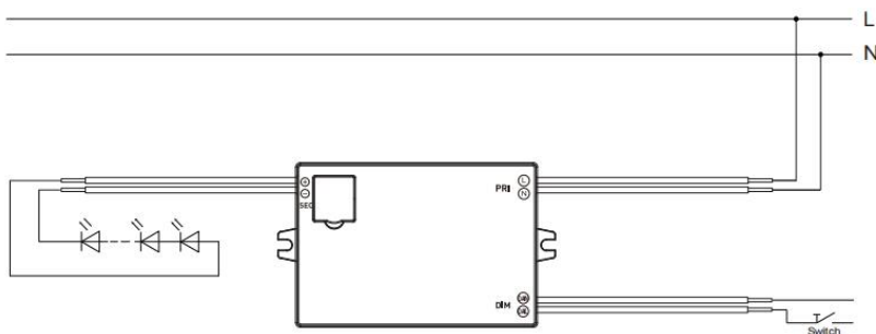
Wiring Diagram (Corridor Function)
